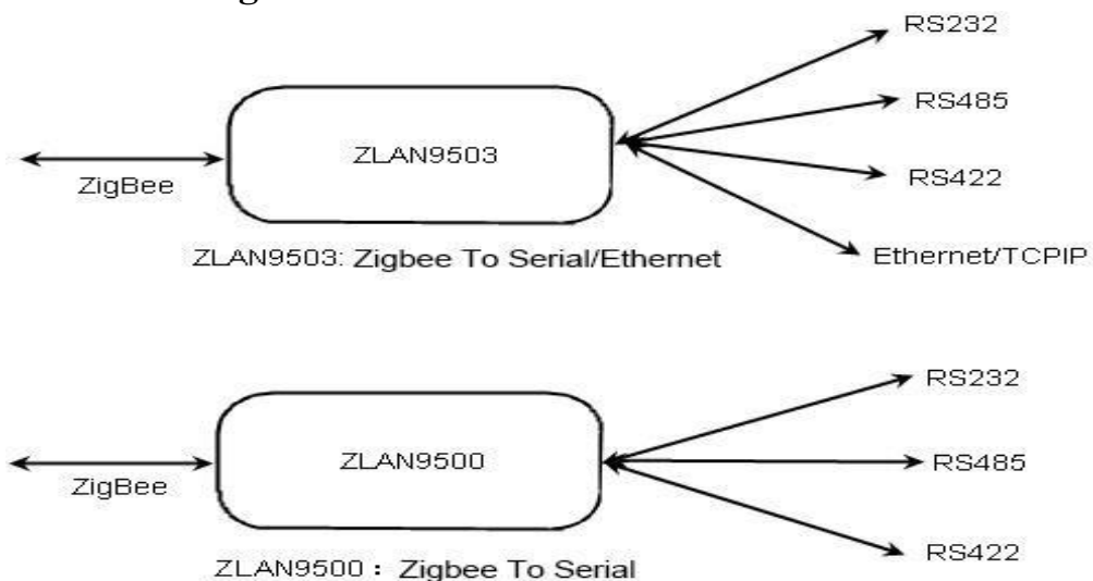
Figure 2 Function Diagram
