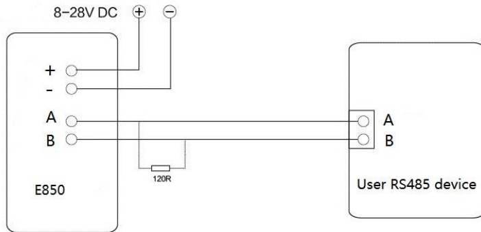
RS485 connection
